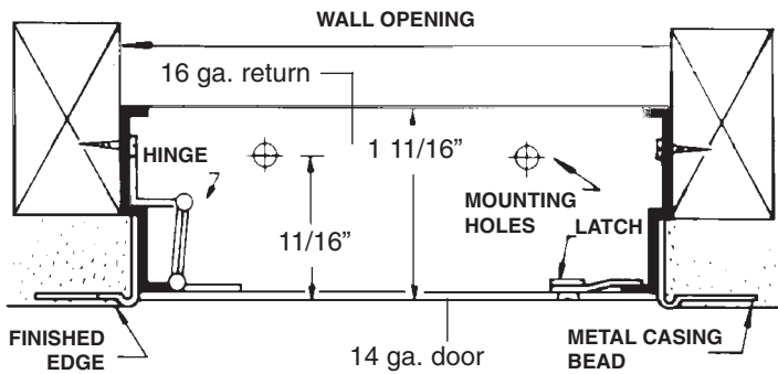
SECTION DETAIL
