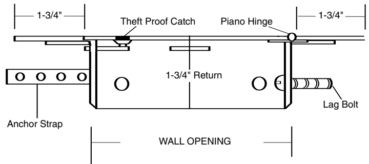
SECTION DETAIL
