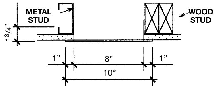
SECTION DETAIL
