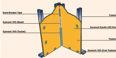
Inside Corner
