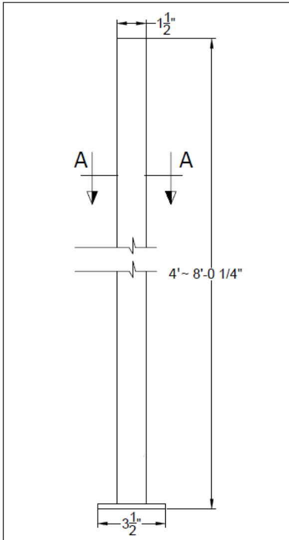
1 ANCHOR ELEVATION
